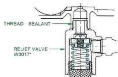
Fig. 2 - Control Valves
