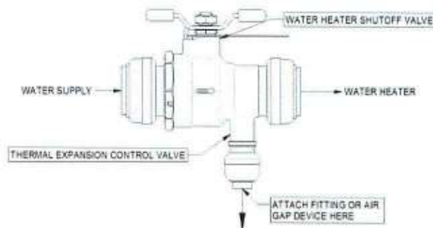
Fig. 1 - Sample Orientation
